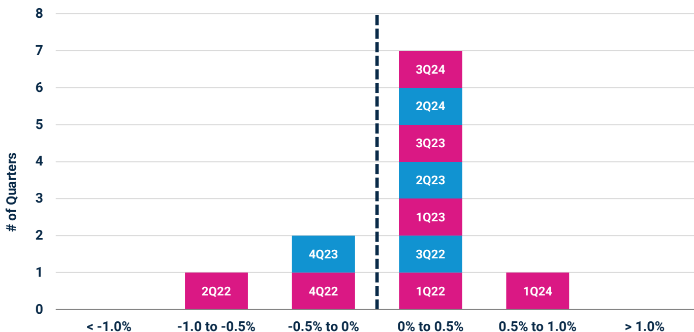
Harbor Core Plus vs. Bloomberg US Agg Bond TR USD Histogram of Quarterly Excess Returns March 2022 - September 2024
